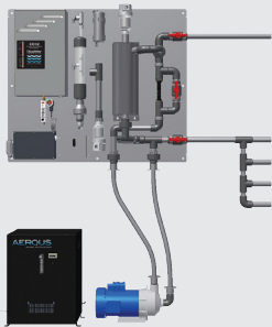
CIP-Panel Mount
